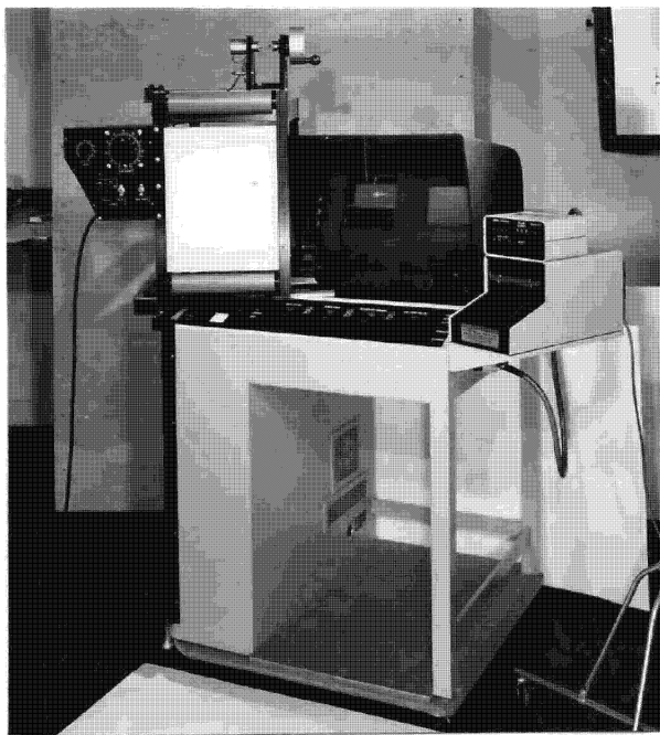
Figure 53 - Video Color Analyzer
