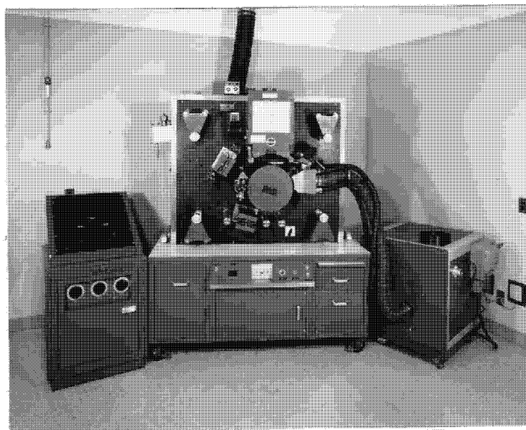
Figure 54 - Rainbow Printer
