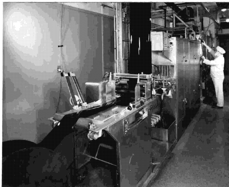
Figure 24 - Yardleigh Processor
