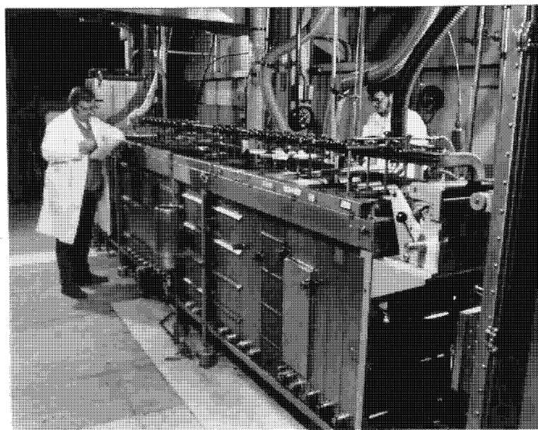
Figure 48 - Grafton Processor
