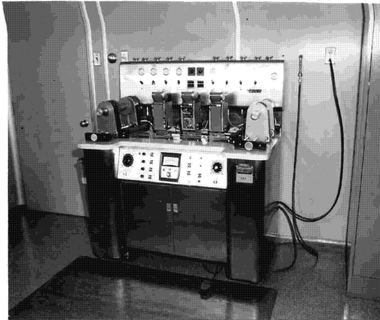
Figure 52 - Unimak Film Titler
