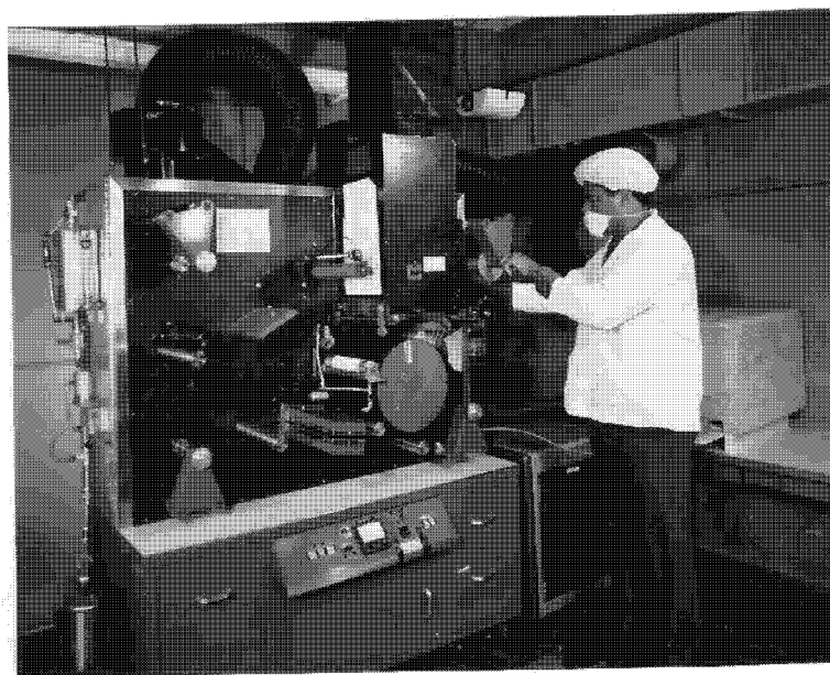
Figure 54 - Rainbow Printer
