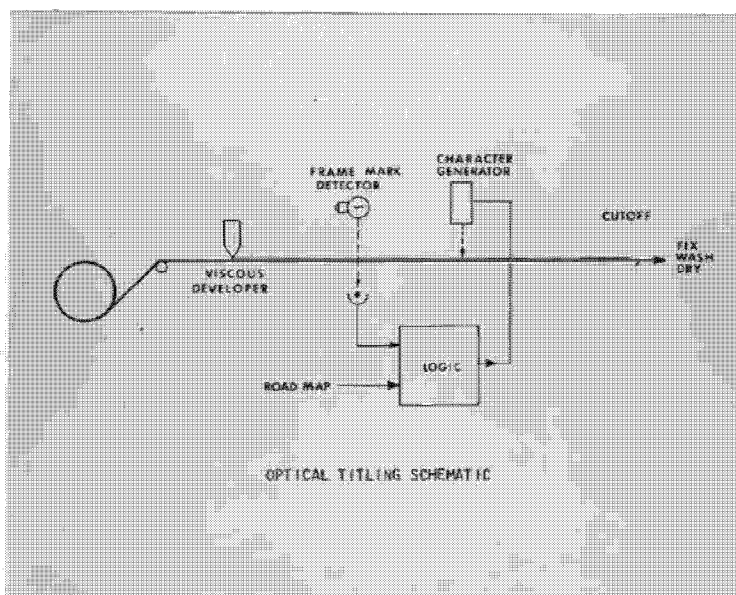
Figure 27 - Optical Titling Schematic
