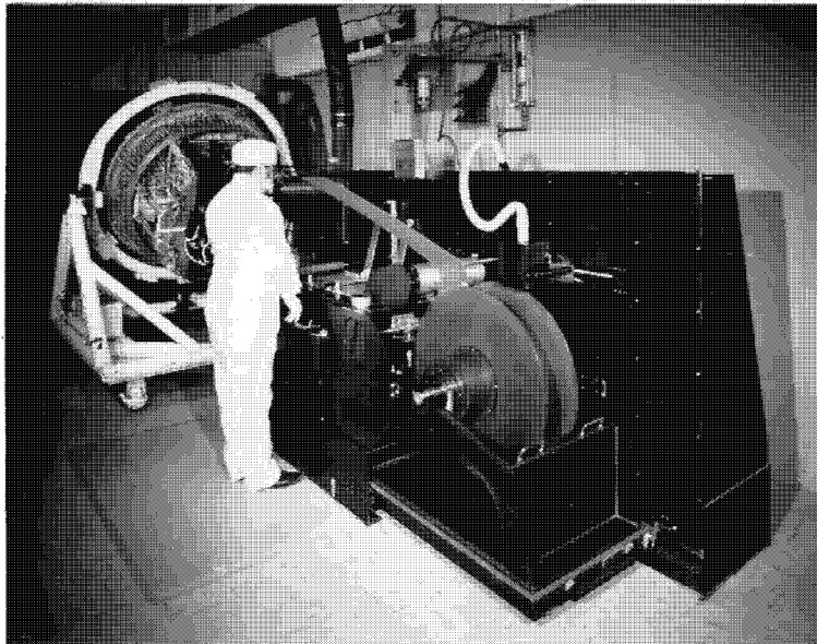
Figure 22 - Hexagon SRV Interfaced with Presplice Complex
